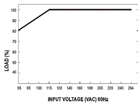
Static characteristic
